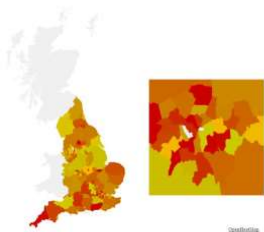
Figure 7 Full network DEA model – node 1
