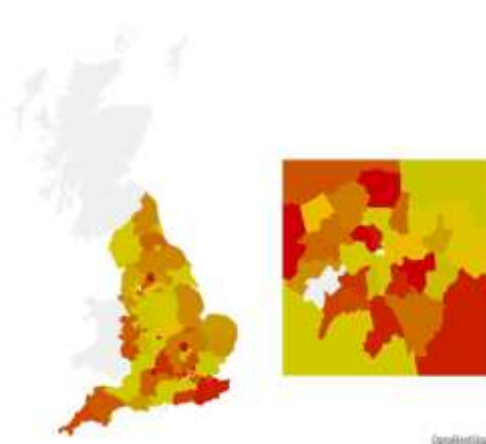
Figure 6 Full DEA model
